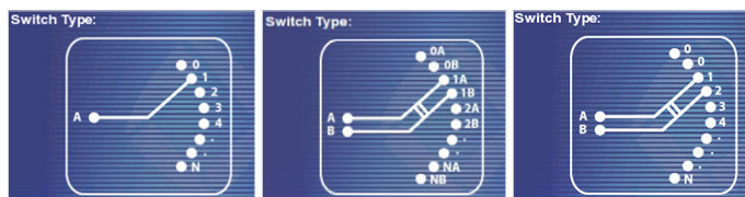
Figure 7. Single common (1C type), duplex (2D type), and dual parallel (2E type)
