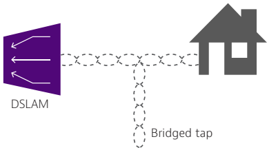
Bridged taps can impact DSL performance
