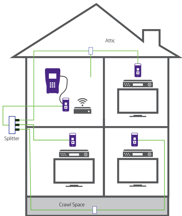
Coax home network under test with SmartIDs
